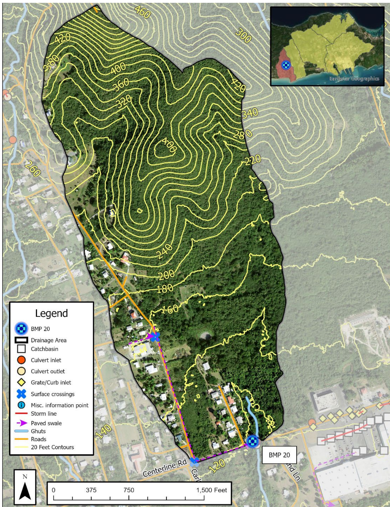
Figure 80. BMP 20's drainage area and its associated infrastructure
